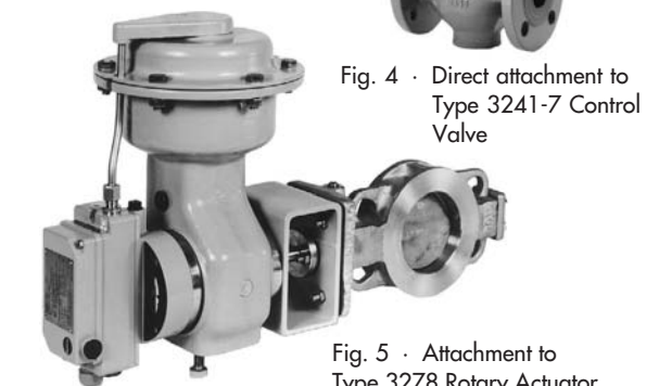
Fig. 3 · Attachment acc. to IEC 60534 (NAMUR)
